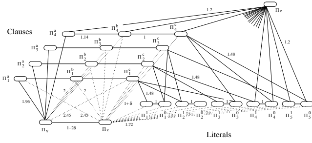
Figure 4: The graph G_I for instance I = (x_1 \vee x_2 \vee \bar{x}_3) \wedge (\bar{x}_1 \vee x_3 \vee x_4) \wedge (\bar{x}_1 \vee x_2 \vee x_5) \wedge (x_3 \vee x_4 \vee x_5) . Each cluster contains k peers with pairwise distance of \epsilon . \delta is an arbitrarily constant such that \delta > \epsilon > 0 .
