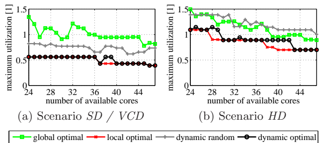
Figure 11: Comparison of the maximum core utilization for different numbers of available cores and different optimization strategies. The dynamic optimal mapping strategy represents the hybrid scenario-based mapping optimization strategy proposed in this paper.
