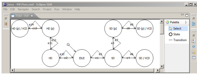
Figure 9: FSM of the PiP software. Paused applications are indicated by a (p) following the application’s name.
